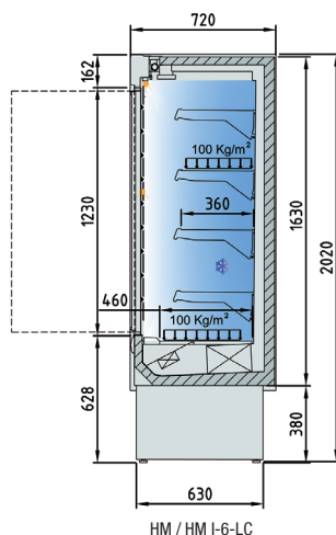
HM / HM I-6-LC
